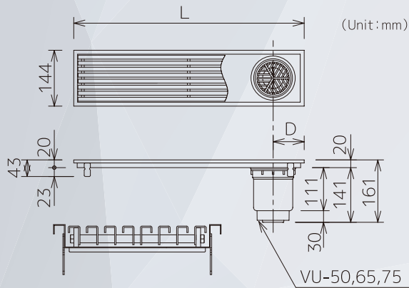
Drain Outlet vertical drain Trap
