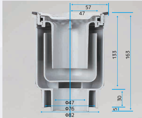
Inner Dimension
