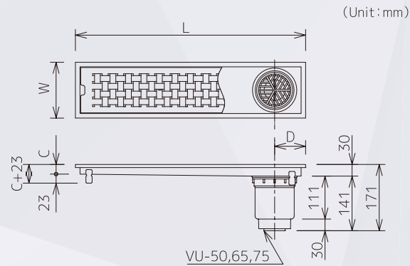
Drain Outlet horizontal drain Trap
