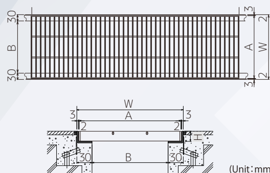
Plain type
