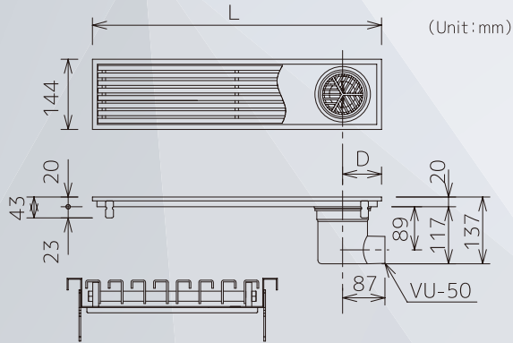
Drain Outlet horizontal drain Trap
