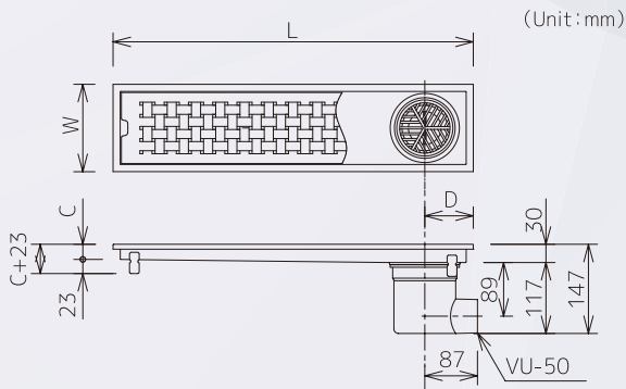
Drain Outlet horizontal drain Trap
